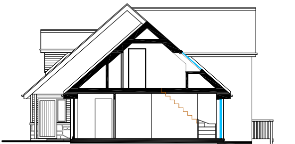
Section BB @ 1/200
