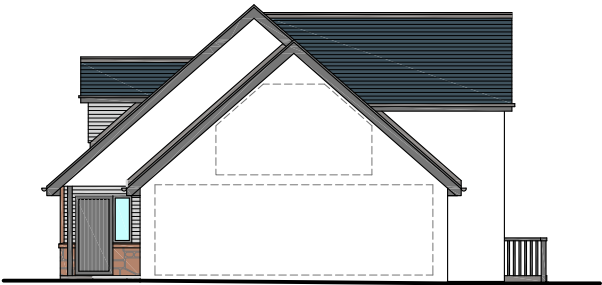
North West Elevation @ 1/200
