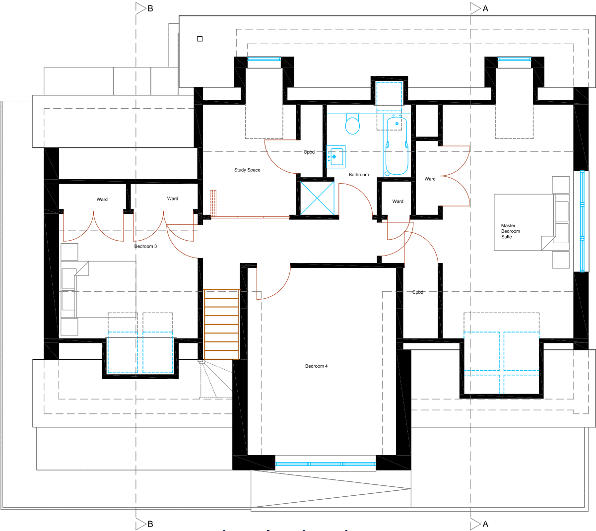
Plot 1 First Floor Plan @ 1/100
