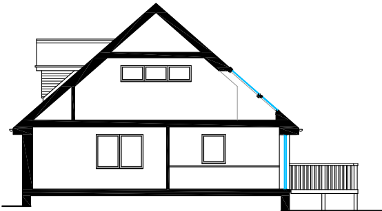
Section AA @ 1/200
