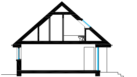
Section BB @ 1/200
