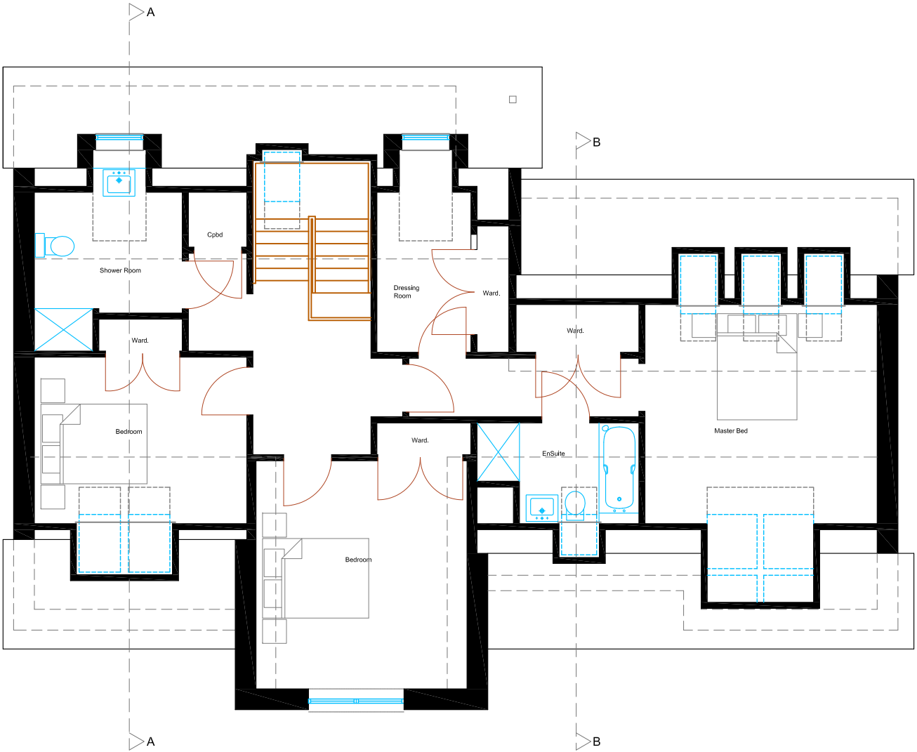
Plot 2 First Floor Plan @ 1/100
