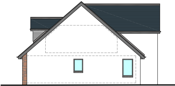
North West Elevation @ 1/200
