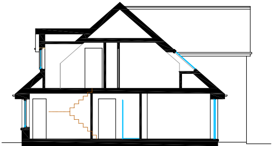
Section AA @ 1/200
